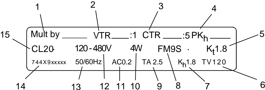
Figure 3-3. Lower Nameplate
